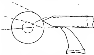
FIG. 301. DETAIL OF PARTING TOOL POSITIONS.
